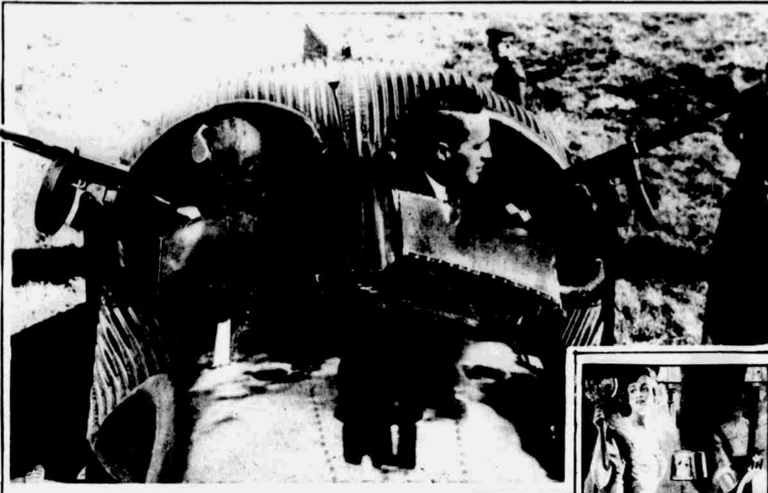
A GUN PIT ON THE AERIAL TANK. Two of the thirty machine guns of the JI-2, an all-metal armored military monoplane which made an initial non-stop flight from Washington to New York in two hours. The "engine of death" will fire 3,000 shots (.45 caliber) in four seconds while flying at 140 miles an hour. H. A. R. from Paul Thompson.
