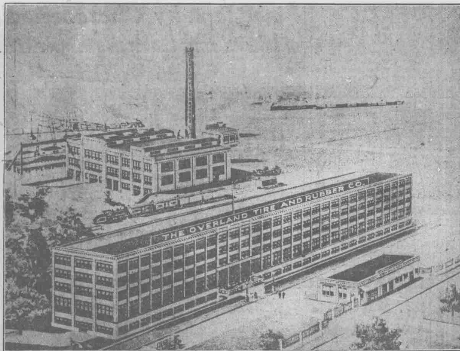
The Overland Tire and Rubber factory will be 75x400 feet, five stories in height, giving us 150,000 square feet of floor space. Back of the factory will be a power house equipped to supply 2,500 horsepower.
