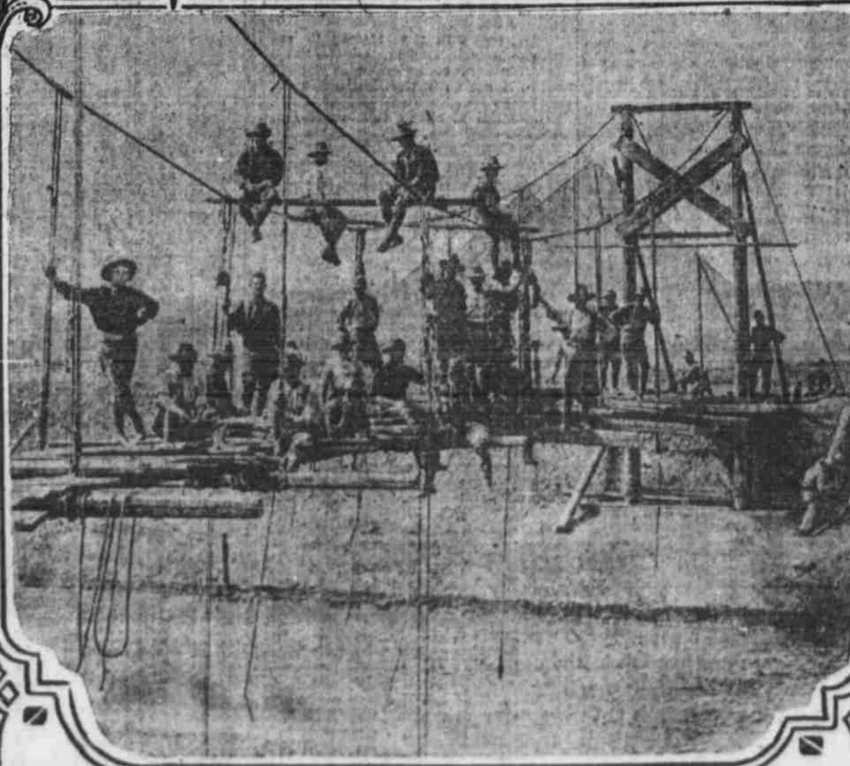
Military suspension bridge in course of construction, over canal near Australian camp at the pyramids
