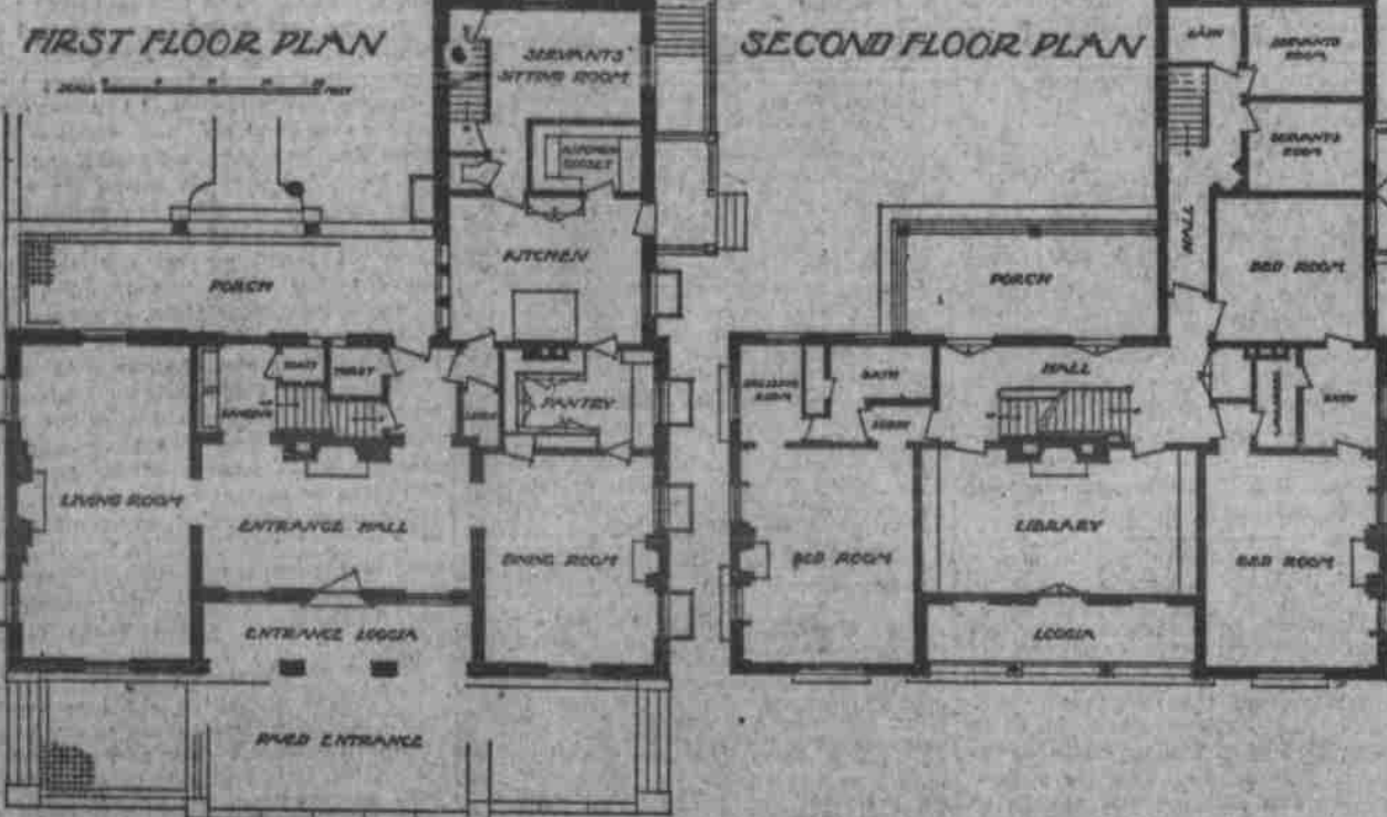
HOUSE AT HERKIMER, N.Y. CHARLES C. GRANT, ARCHITECT
