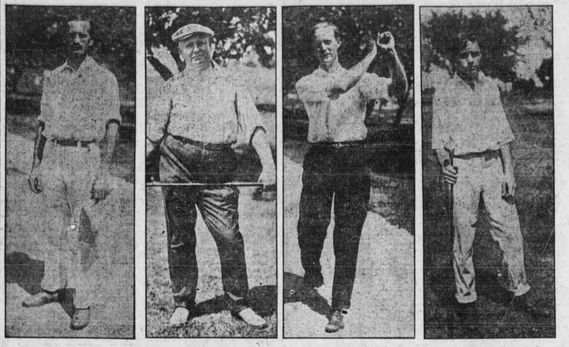
DR. HOLLISTER, in Semi-Finals. DR. SUMNEY, Champion. SPRAGUE ABBOTT, Runner Up. BLAINE YOUNG, in Semi-Finals.
