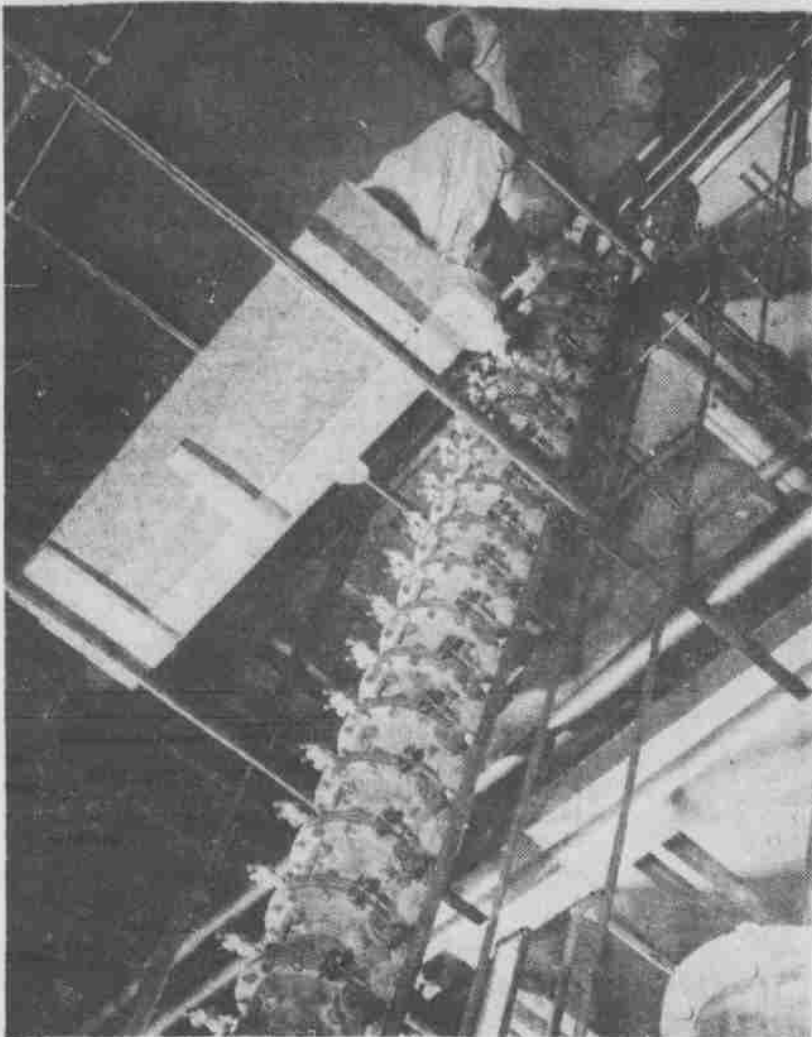
PRIDE OF THE CHEMICAL engineering department is this recently completed fractionation column, which will be in operation the night of Engineer's Week Open House. The unit is about 24 feet high and built of copper and brass. It is used in the fractional distillation of petroleum products. The crude oil is placed in the reflux chamber and as it distills, the gasoline, kerosenes, fuel oils, organic solvents and oils are separated. It is very similar to the kind that large oil companies use, but it is built on a smaller scale. Ed Galloway, a Chem E, is on the platform.
