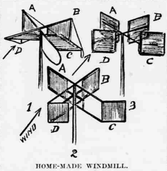
HOME-MADE WINDMILL.
