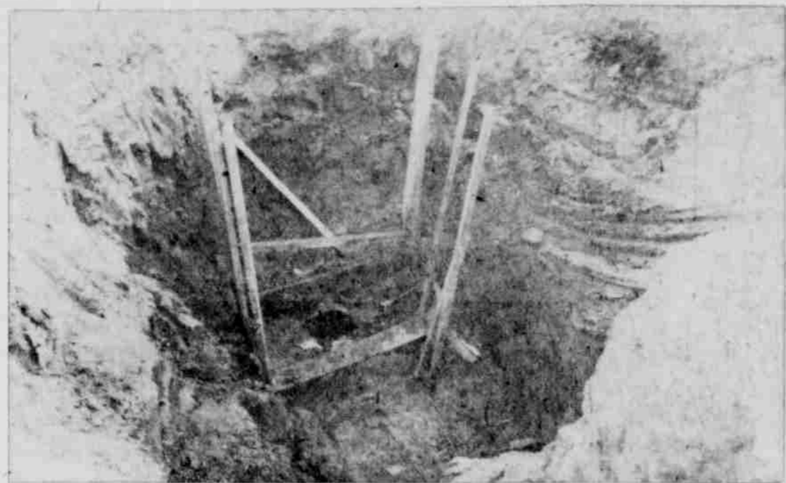
RAILROAD CROSSED — Shown above is the west end of the 24-inch cast iron sewer pipe which was rammed beneath the Burlington Railroad right-of-way here. It will be the outlet sewer's connection with the sewage treatment plant being built below the tracks. The pipe is 162 feet long and was pushed through with a hydraulic ram with about 175 tons pressure at a depth of about 21 feet.
