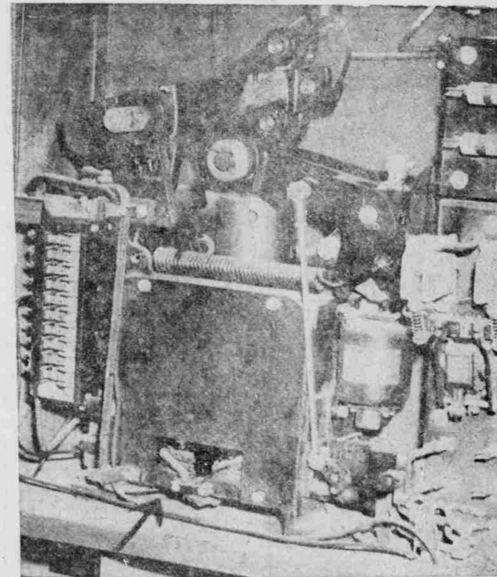
Pictured above is one of the giant switches that melted down from terrific heat. Arrow points to molten insulation that oozed from the bottom of the switch. A circuit to Bellevue passes through this line and was soon back in service when employees pulled the switch back in position by a manually operated lever after the automatic throw-out was destroyed.—Journal Photos.
