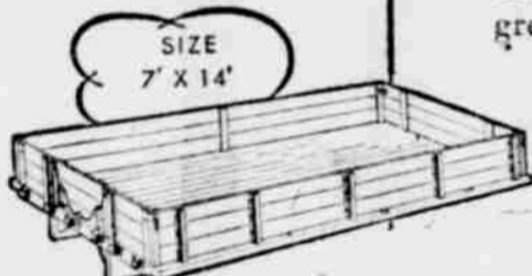
Here's a sturdy, useful wagon box for general hauling, with tractor or team. Capacity, level full, 90 bushels of small grain.
