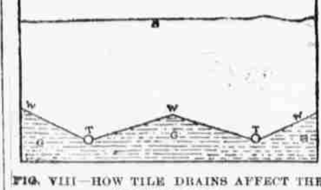
FIG. VIII.—HOW TILE DRAINS AFFECT THE WATER TABLE.
