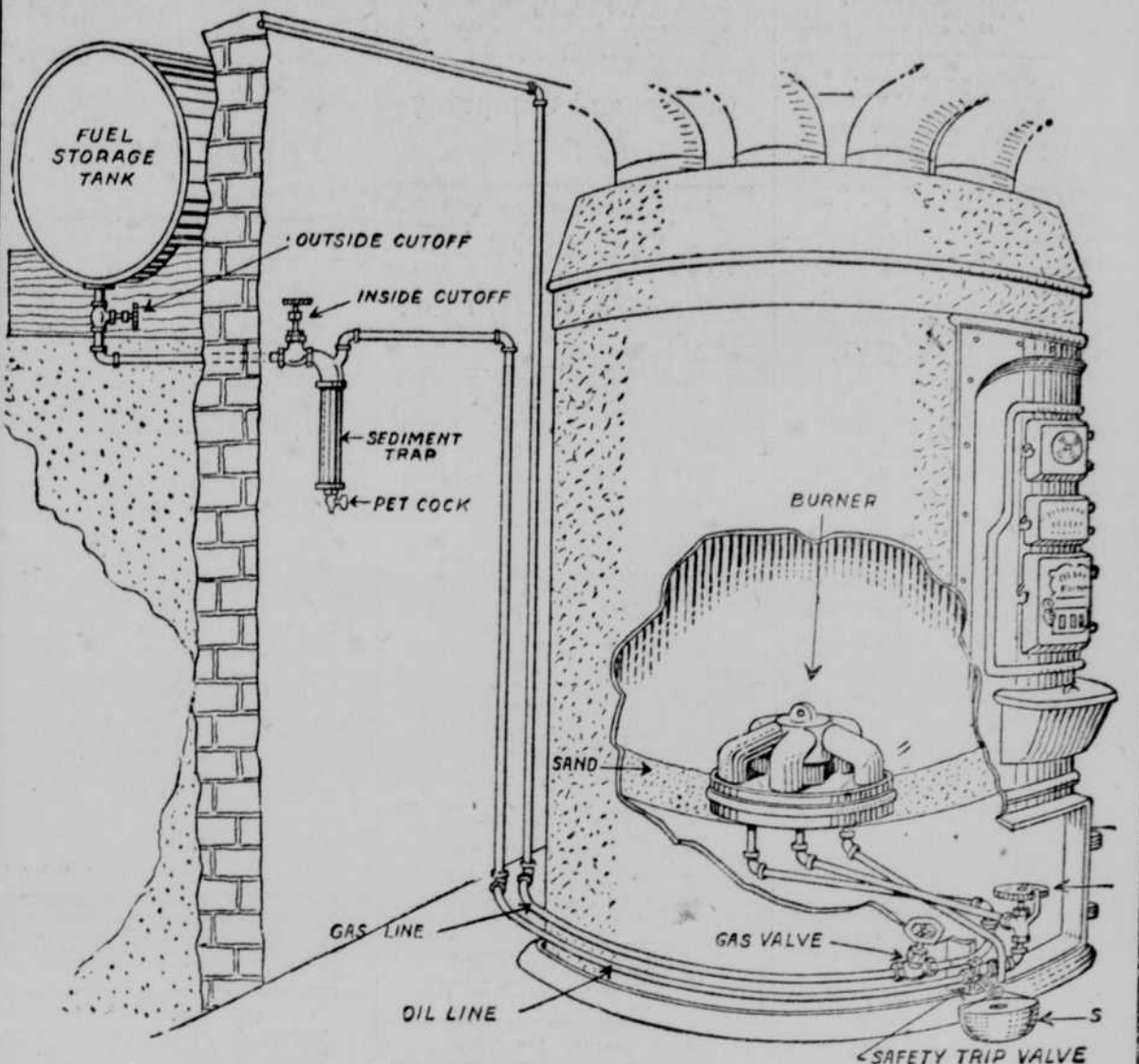
Drawing Showing Complete Installation
