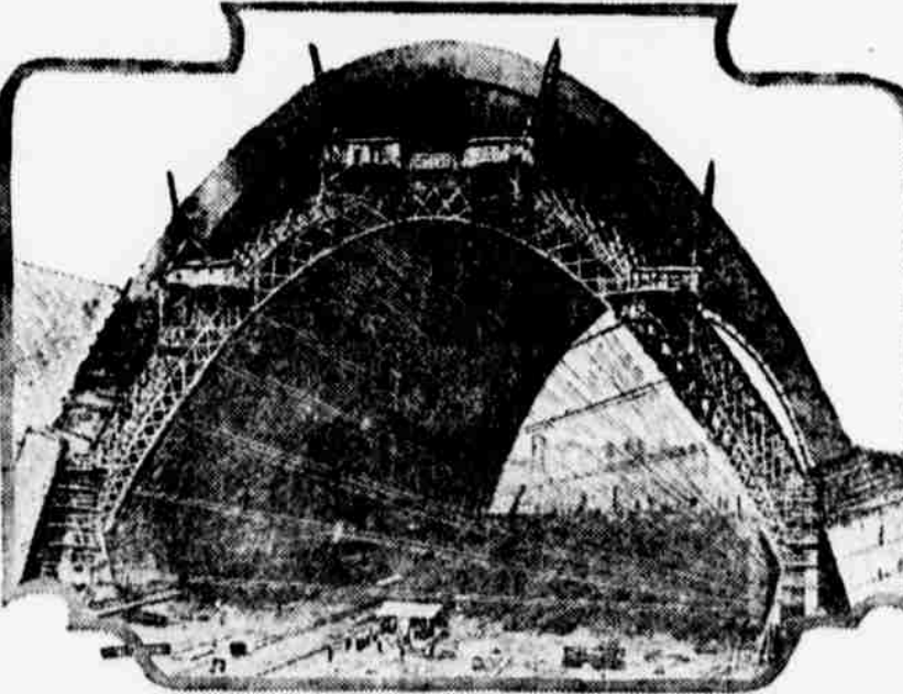
A new epoch in construction is marked by the nearly completed hangar at Orly, near Fontainebleau, France. This hangar will be the largest in the world when finished.
