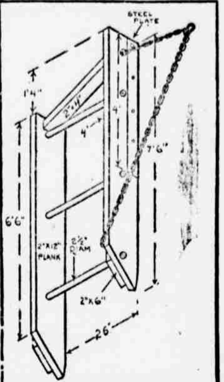
Plan of Plank Road Drag.
