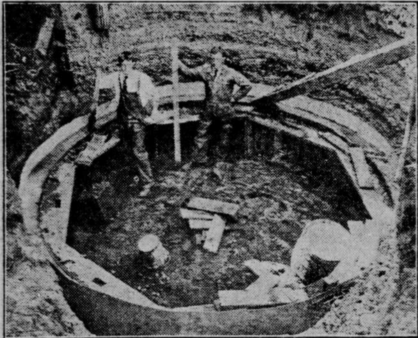
Students Constructing a Concrete Silo.
