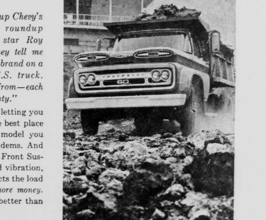
Chevy's hefty 261-cu.-in. Jobmaster 6 is a big reason for the outstanding popularity of Series 60 middleweights.
