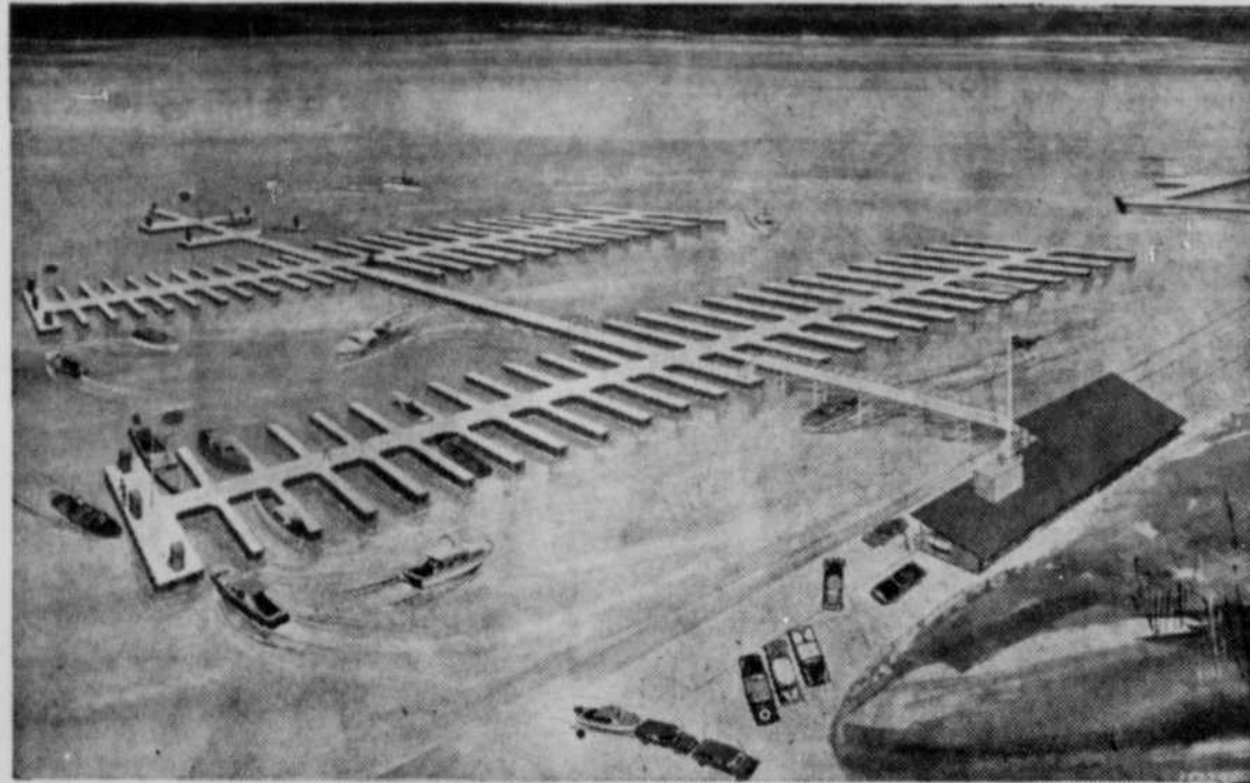
A new 200 slip, all steel, floating marina has been completed at Picktown, S. D., and is now accommodating boats using the Fort Randall Reservoir.
