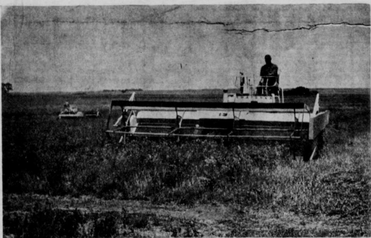
Although this is not a new invention it is one of the first ones we've seen at work in Holt county hay fields. It's a mower, hay conditioner combination. The machine cuts a 16 ft. swath, runs the hay through crimping rollers and automatically windrows it. University of Nebraska agricultural experts say nearly twice as much feed value is realized from this type of operation. Two of these machines are being used now on the L. D. Putnam ranch northeast of O'Neill.
