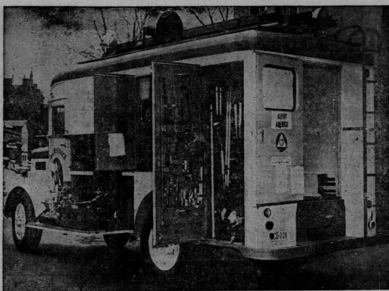
'CALAMITY JANE,' the Federal Civil Defense Administration's rescue truck, packs a wallop from debris. The $9,000 truck contains 300 pieces more potent than its namesake's six-shooters of rescue equipment of 99 different types.
