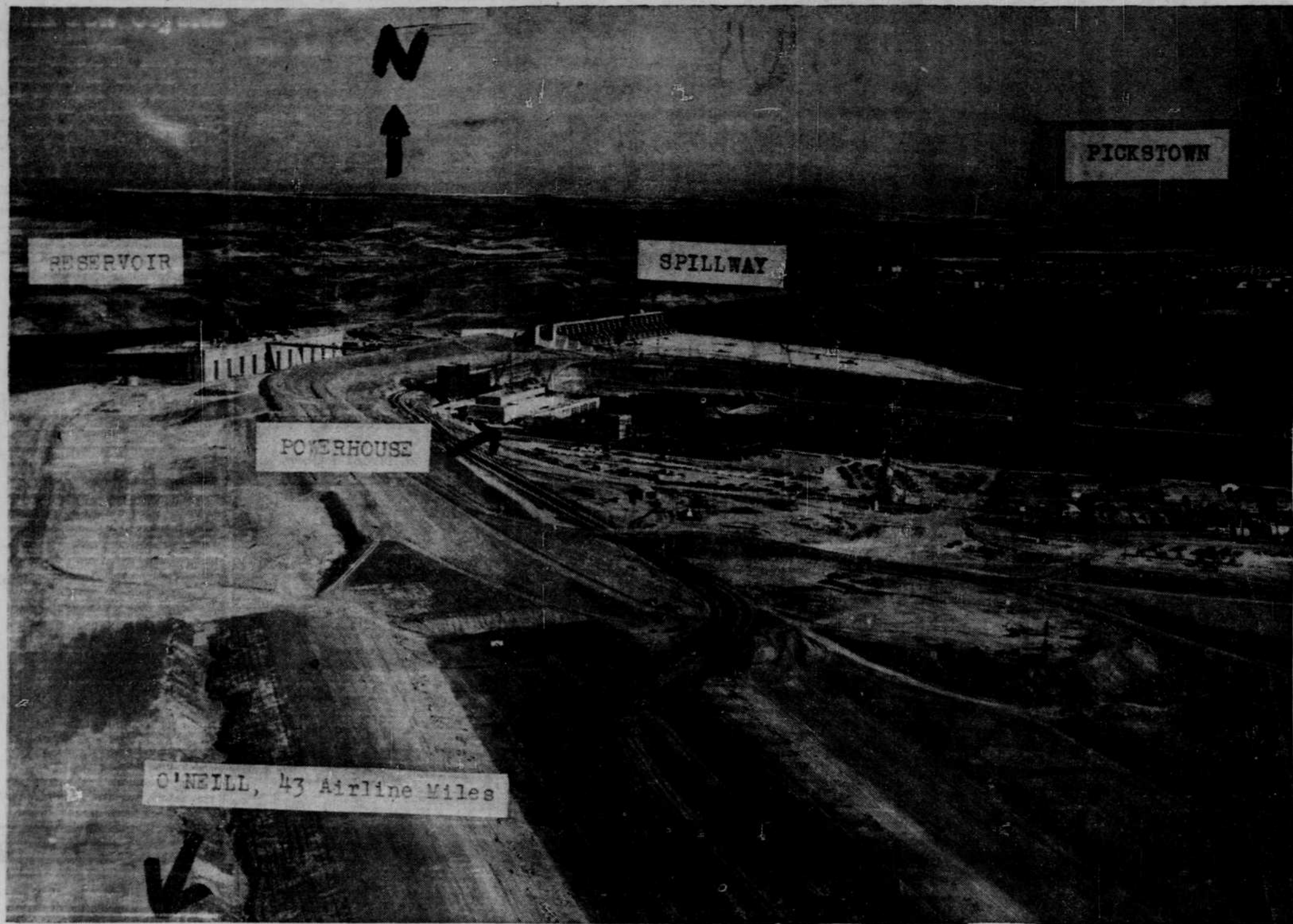
Looking along the earth embankment of Ft. Randall dam, being built by army engineers across the Missouri river at Pickstown, S.D. Ft. Randall is the nearest to completion of five mainstem developments. Now three-fourths finished. Ft. Randall was started in 1946. At the bottom of the photo, earth-moving equipment places fill in the final section of embankment. Twenty-seven out of an ultimate 28-million-cubic yards are already in the dam. The low white-appearing building to the right of the
