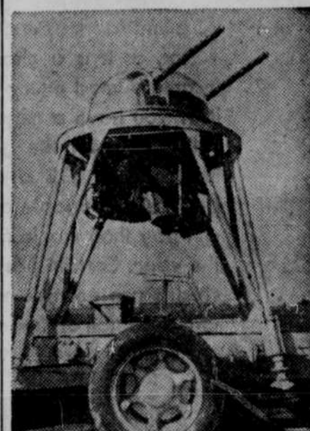
This movable contraption is an airplane gun turret without the airplane. Trainees of the U. S. Naval Gunnery school in San Diego, Calif., fire round after round of ammunition from this perch.
