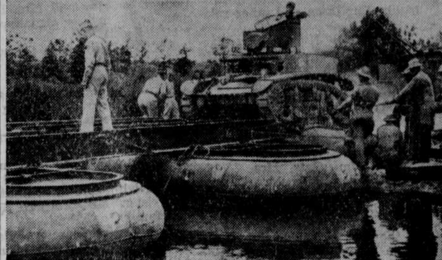
Officers of the 16th engineers, Fort Knox, Ky., have devised a pontoon bridge capable of transporting the heaviest tanks. Rubber pontoons are used instead of wooden floats. Photo at top shows pontoon with men ready to move it into place. Below is a section of the completed bridge showing a light tank climbing the rails to cross the bridge. The light tank weighs approximately eleven tons.
