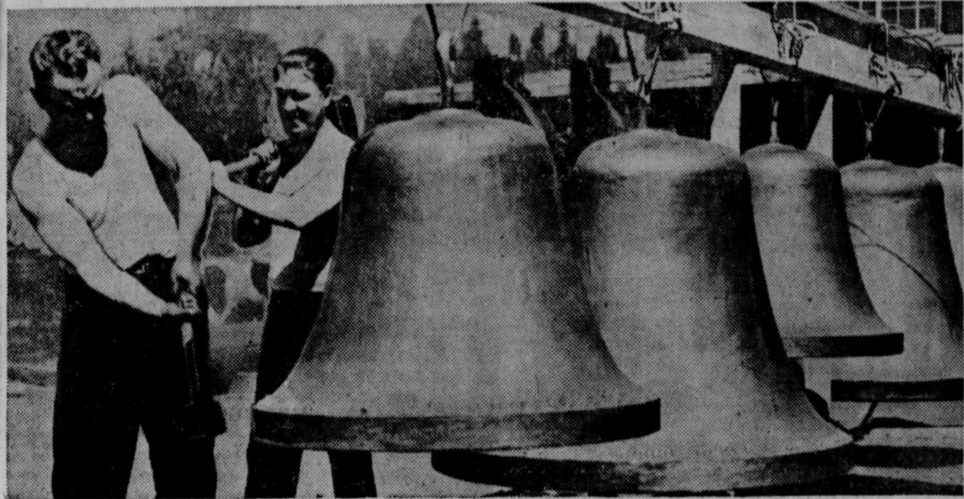
One of the many safety measures to be installed on the gigantic San Francisco-Oakland bay bridge is a group of five huge bells, one for each tower and the central anchorage. The bells, largest ever made in western America, have been undergoing tests in a San Francisco foundry for tone and carrying power. Workmen with sledge-hammers are seen pounding them. Each bell is of a different pitch and when installed they will resound over the bay like giant chimes.
