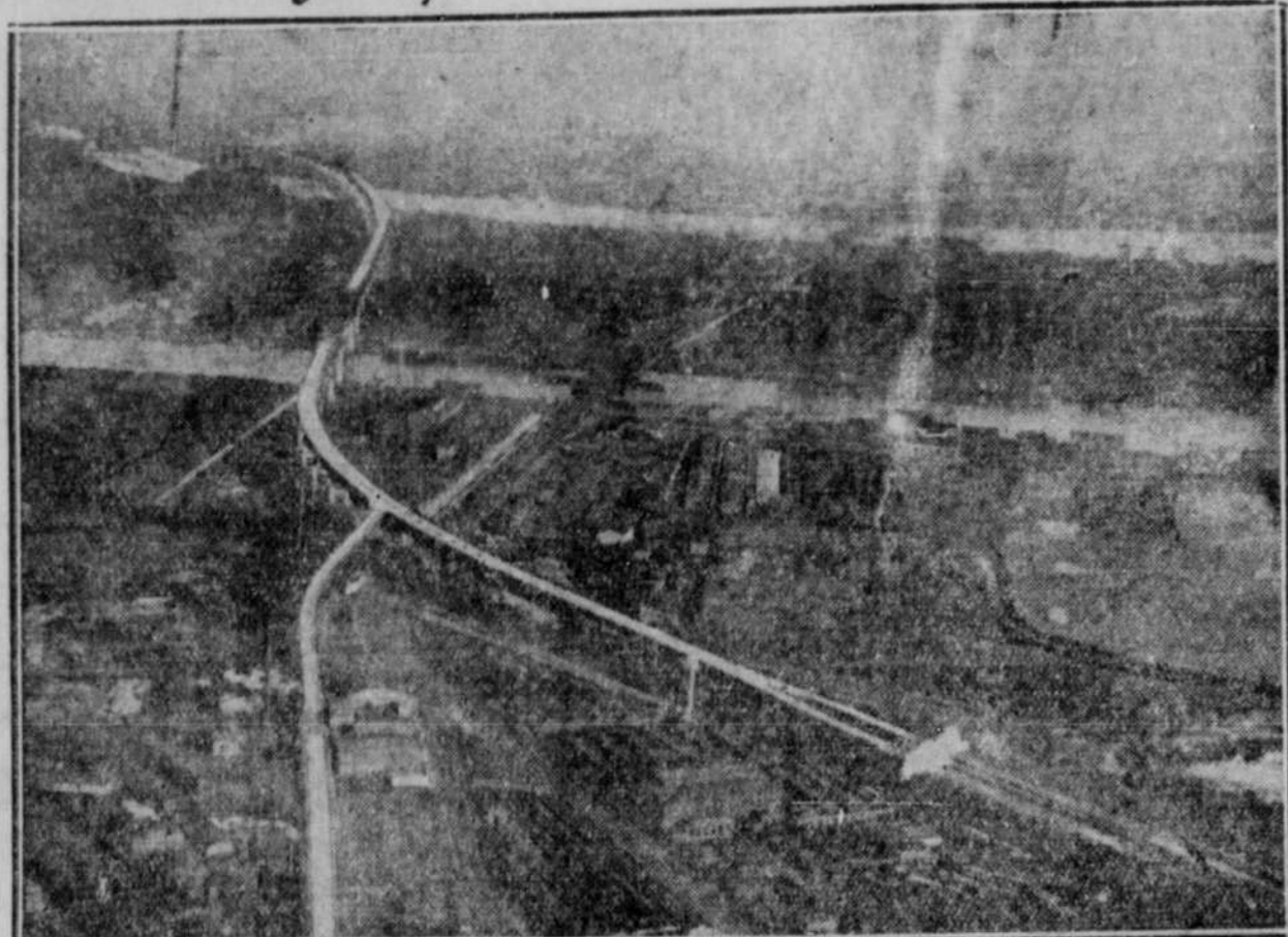
Here is a birdseye view of the new three-mile elevated highway which connects the Hudson Tunnel from New York with the three New Jersey cities—Jersey City, Newark and Kearney. The road is regarded as one of the greatest engineering accomplishments of its kind in the world. Its completion ends four years of intensive labor. It cost $18,000,000 to build and was designed by Col. H. W. Hudson.
