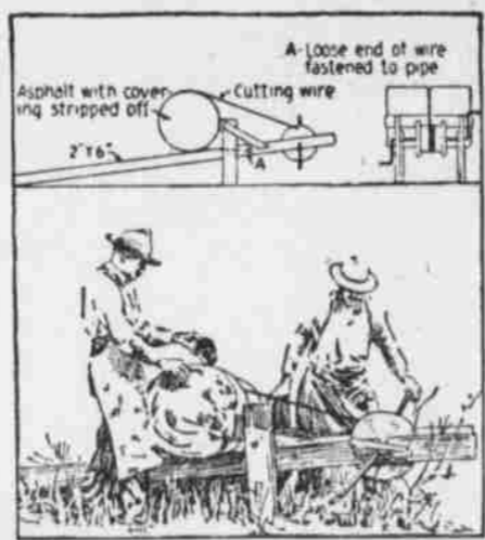
Cutting Asphalt Taken From Barrel With a Wire Drawn Through It With a Windlass.
