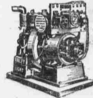
Lalley-Light is a complete unit—engine and generator—with 16-cell storage battery. It supplies ample electricity for lights, water pump, washing machine, squeezer, cream separator, faning mill, iron, etc.
