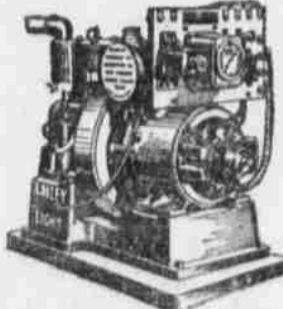
Lalley-Light is a complete unit—engine and generator—with 10-cell storage battery. It supplies ample electricity for lights, water pumps, washing machines, scrapers, cream separator, fanning mill, iron, etc.
