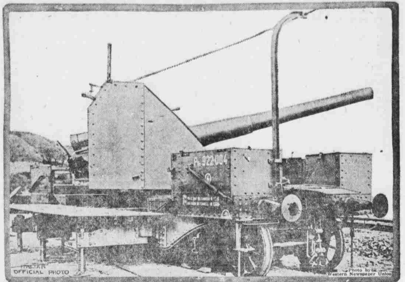
This is one of the huge naval guns with which the allies hammer the Austrians on the Italian front.
