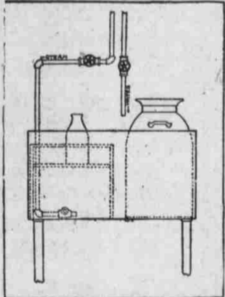
Sink Arranged for Pasteurization of Milk.
