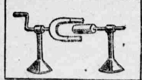
Plan of Magnetic Transmission.
