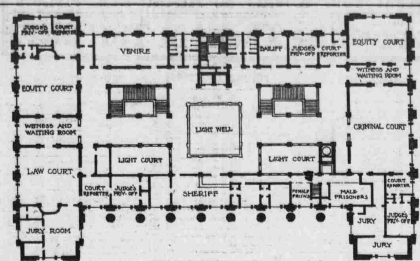
DOUGLAS COUNTY COURT HOUSE FOURTH FLOOR PLAN
