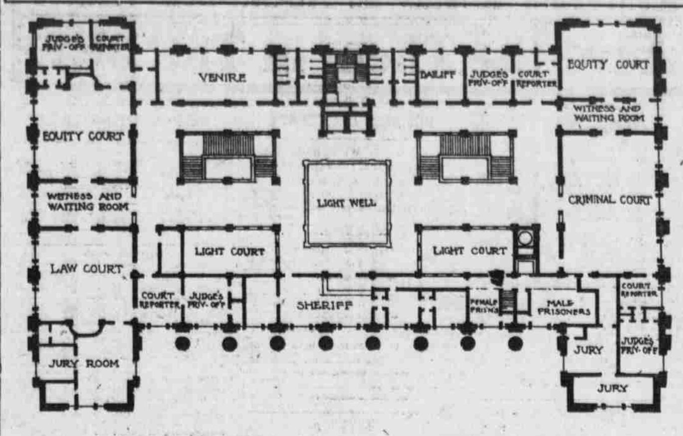
DOUGLAS COUNTY COURT HOUSE FOURTH FLOOR PLAN
