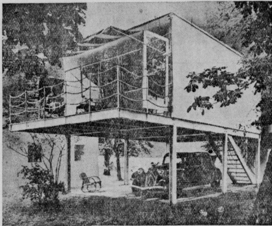
This unusual week-end house was erected on six legs at a vacation point near Stockholm, Sweden. The open space under the house provides space for automobiles. Steel I-beams form the supports and main frame for the structure. The house is similar in principle to modernistic dwellings which have been introduced into the United States in recent years. The structure is prefabricated and can be readily assembled on the lot.
