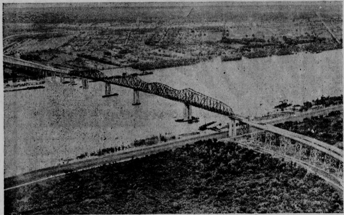
With pageantry and oratory the Huey P. Long bridge, a $13,000,000 combination rail and highway span, across the Mississippi river three and one-half miles above New Orleans, was dedicated and opened to traffic. It is the longest railway bridge in the world, 4.4 miles over all, and the vertical clearance at extreme high water is 135 feet.
