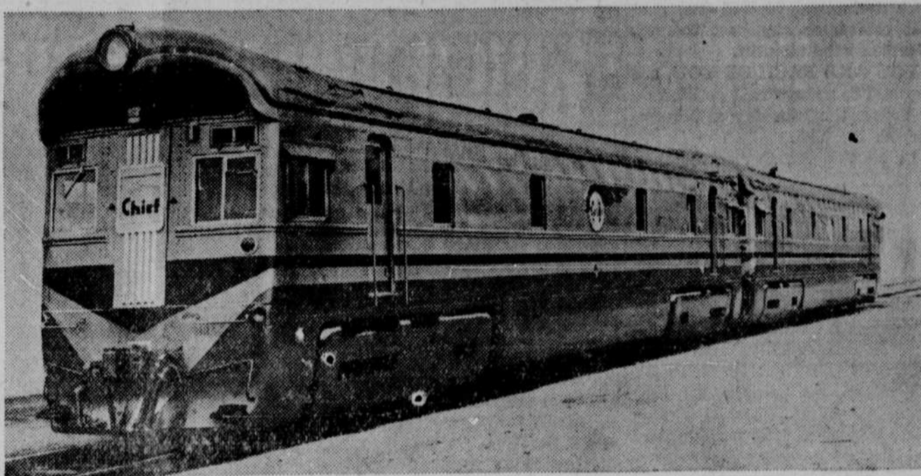
This giant Diesel locomotive built for the Santa Fe railway on tests pulled the road's flier, "The Chief," fast enough to warrant the expectation that the time of that train between Chicago and Los Angeles could be reduced by 12 hours. The engine consists of two identical units which can be operated singly or coupled together. It has an operator's cab and control station at each end. Motive power of each unit is supplied by two V-type, 12-cylinder, high-compression, two-cycle oil engines. The two units provide a total of 3,600 horsepower. It attained a speed of 111 miles an hour.
