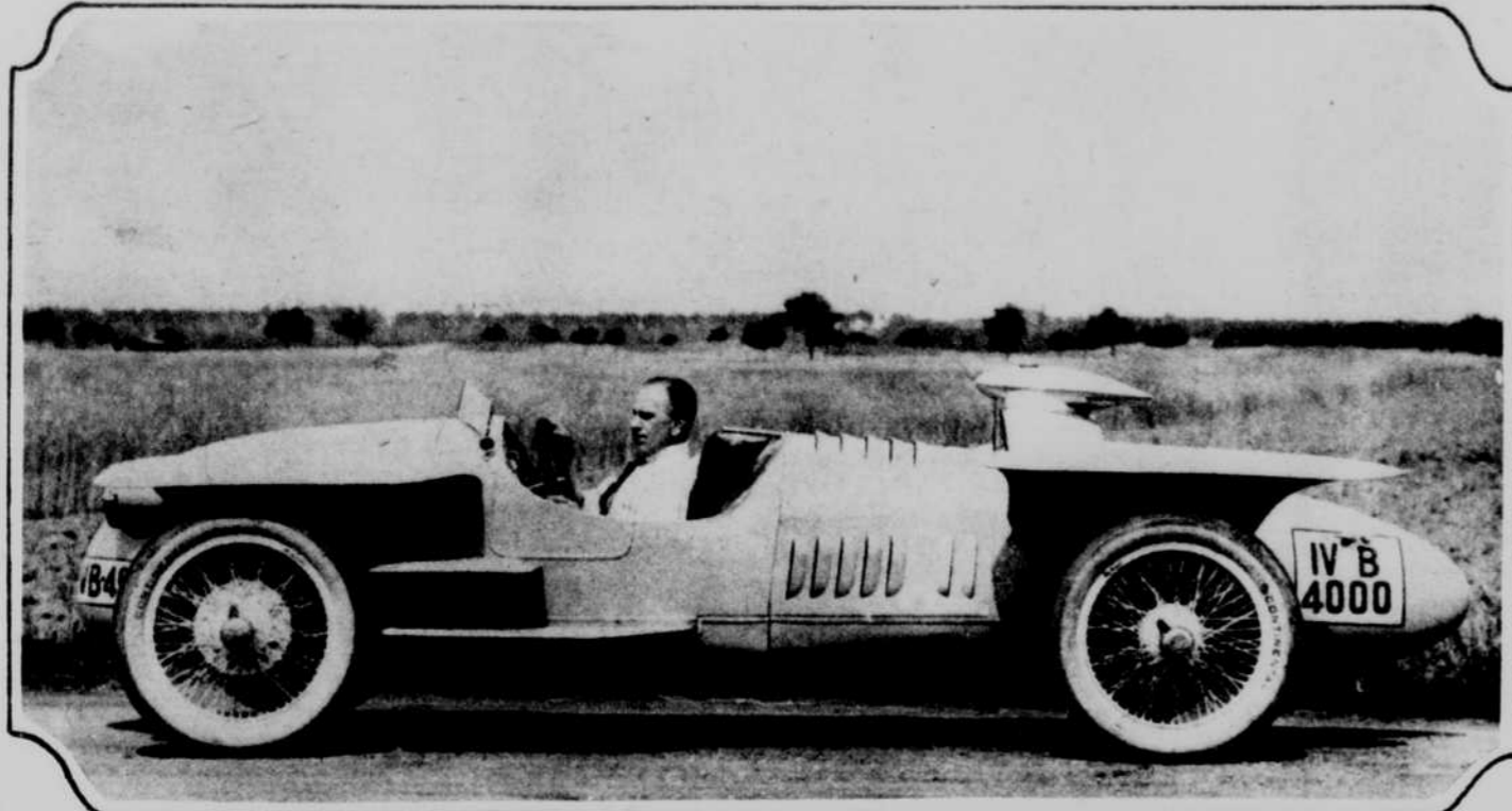
Typical of the racing cars of extraordinary design that have been making their appearance in Europe during the last four years, is this 1924 Benz Rumpier Racer. The power unit, with engine, clutch, gear-box and differential is located at the rear end of the car while the driver's and passengers' seats are located in the front between the axle centers. This new type car bids fair to become the new standard of motor vehicles the world over.
