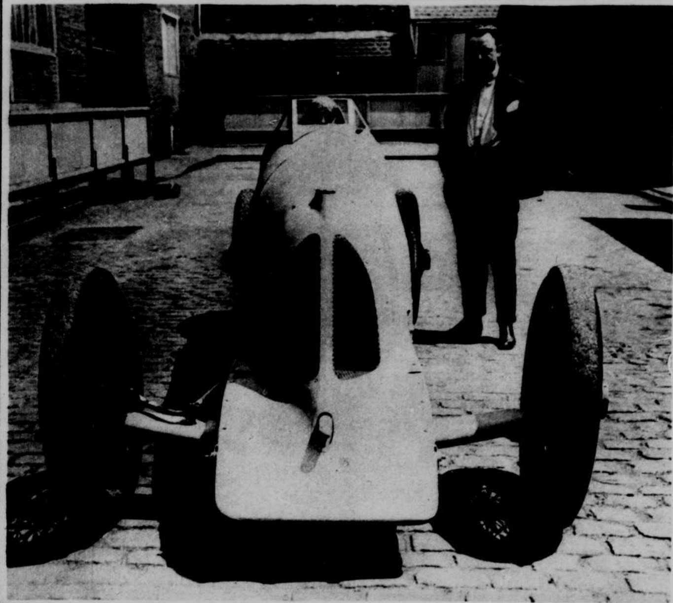
Prince Dejelhdine of Egypt in his racing car which he himself designed to meet America's foremost "speed king's" and which he hopes to make a speed of more than 180 miles per hour. The car has eight cylinders and is 350 horsepower. —Wide World.
