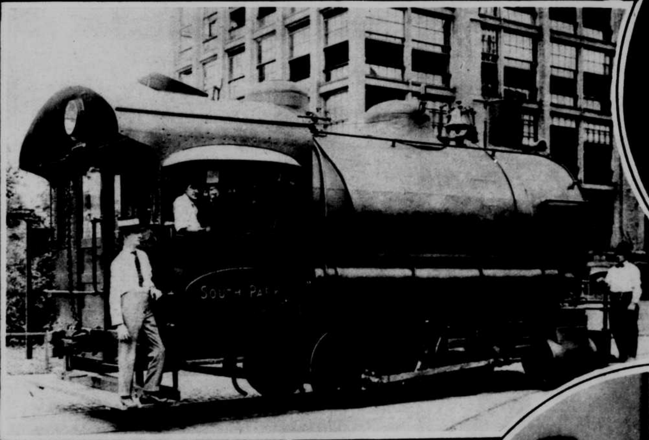
A fireless locomotive that is charged with water and live steam at the boiler plant of the National Cash Register Company, will run for two to three hours without recharging which takes twenty minutes. The test has proven a success and is economical, since it eliminates the necessity of a tender or a fireman. The heavy black smoke which marred the building walls is also done away with. —Wide World.
