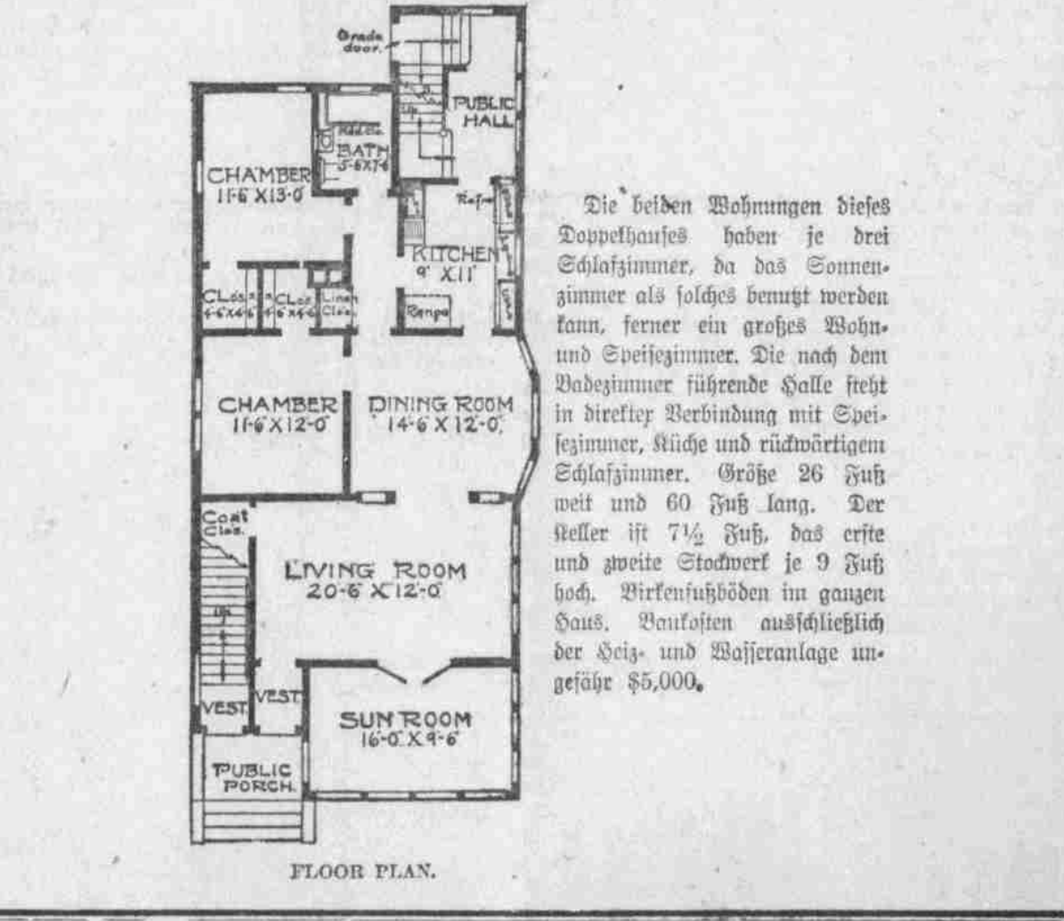
FLOOR PLAN.
