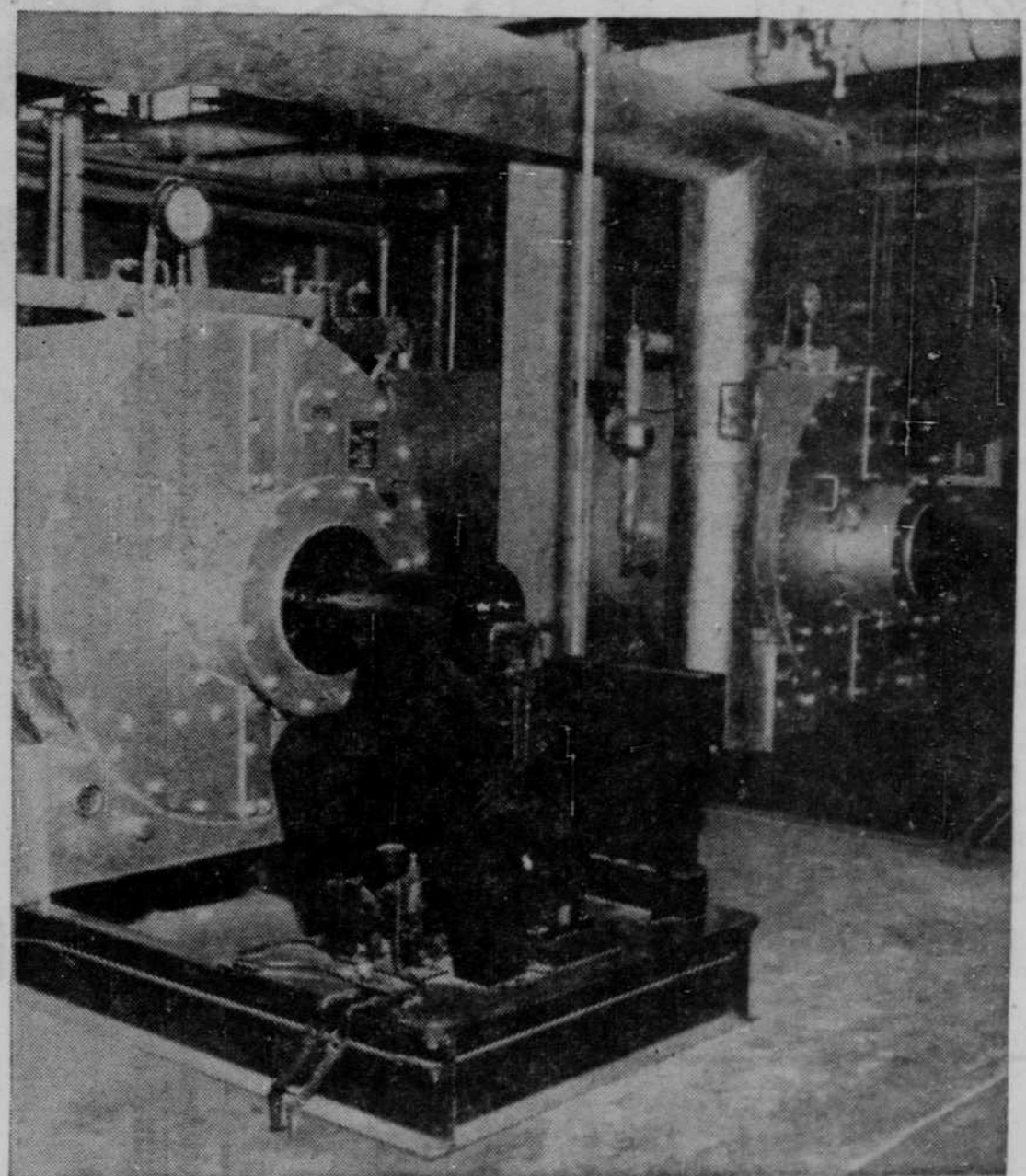
THE HOSPITAL HEATING PLANT
