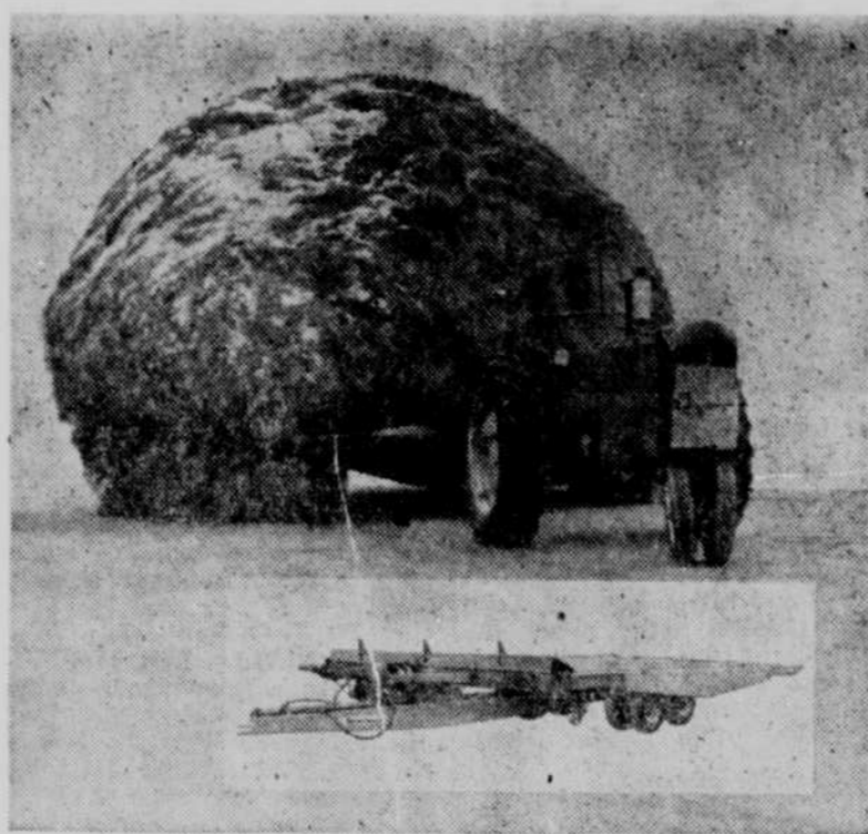
STACK MOVER HAULS 100 TONS A DAY WITHOUT HAND LABOR
