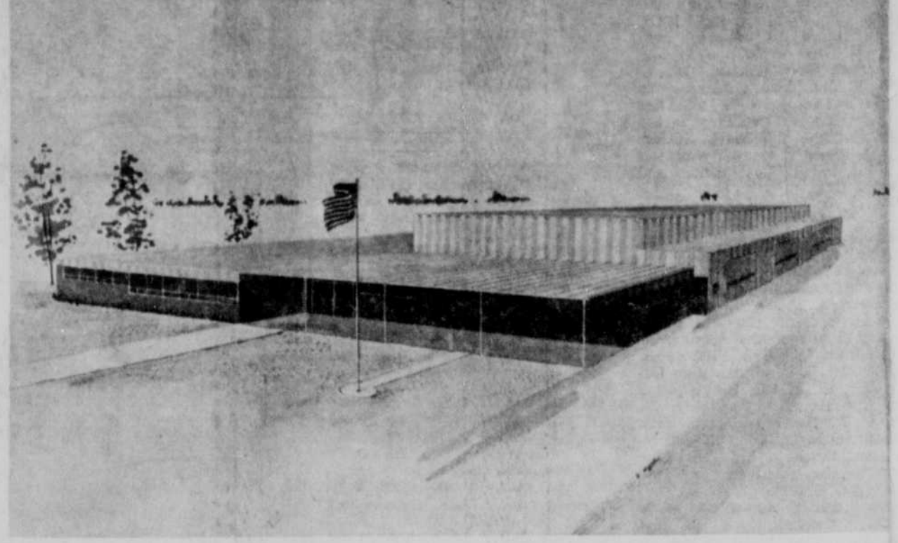
Bids will be let Tuesday for O'Neill's new $90,000 armory shown in the architect's drawing above. The 16,000 sq. ft. building will be used for a drill hall, vehicle and ordnance storage, library and offices. The proposed frameless steel structure will also feature a double panel roof-ceiling system. The O'Neill armory will be the first armory in the U. S. to use the roof-ceiling system.
