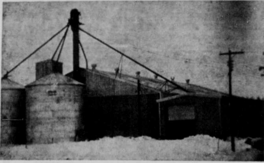
VERDIGRE —The Farmer's Union Grain elevator, completed last December at a cost of $100,000 is built entirely of concrete and galvanized steel with stainless steel bolts. The building is 120 ft. long by 80 ft. wide and 40 ft high and has a capacity of 200,000 bushels and is equipped with a 50 ton scale and aerators. The insulated office building is at right and houses the electronic switch board. Arthur M. Sufficool is the manager.
