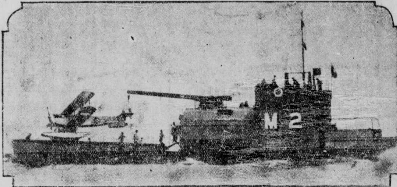
An exclusive photo of England's aircraft carrier submarine M-2, formerly a submarine monitor. The 12-inch gun turret is now used as an airplane carrier. This is the first submarine to be fitted to carry aircraft. (International Newsreel)
