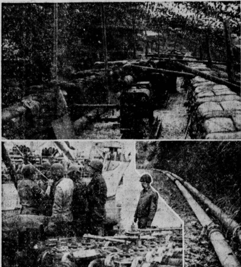
A pumping station, one of many set up along the pipeline carrying vital fuel oil in France. Upper photo shows station carefully camouflaged against air observation. Lower left, ship-to-shore line for unloading petroleum from ships. Lower right, American engineers have laid this gasoline pipeline in France, five miles inland.
