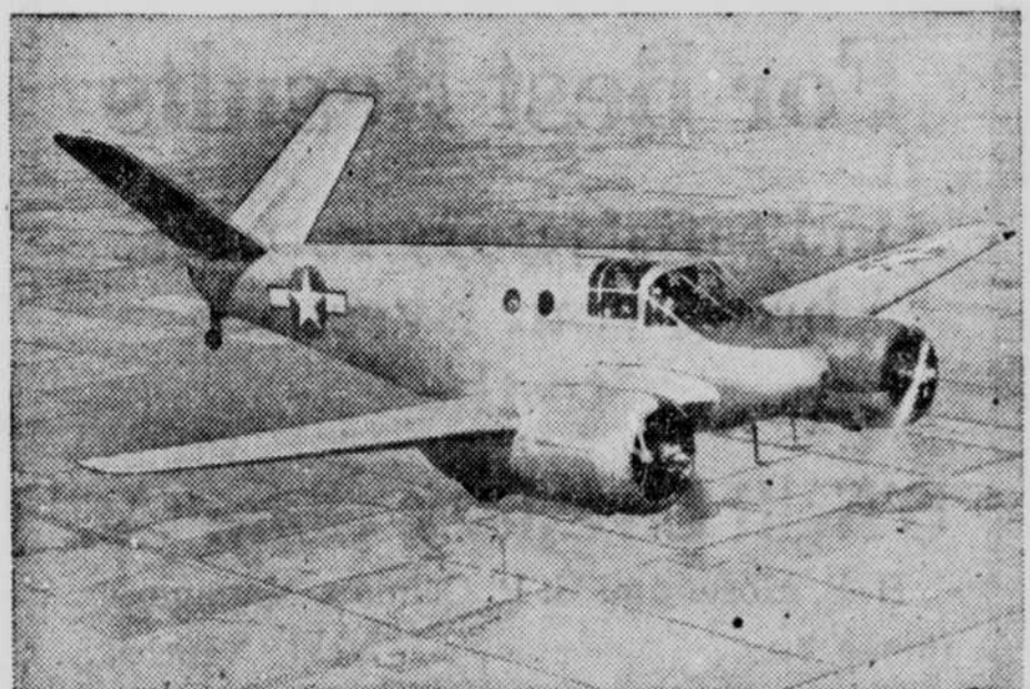
With a V tail, or "butterfly" tail type of only two elements, the latest Beechcraft plane has been successfully tried out. Tests show excellent control and stability characteristics at all speeds. The only trick in the deal is to let the movable control surface know when to act as rudders and when to function as elevators.
