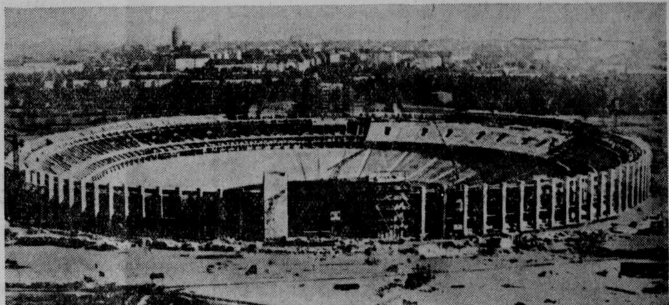
The huge bowl in which many events of the coming Olympic games will take place, is being rushed to completion on the outskirts of Berlin, Germany. This view of the stadium was made from the Fuhrer tower.
