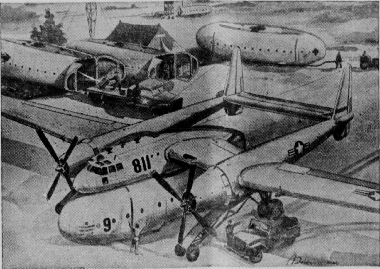
NOW A DETACHABLE FUSELAGE . . . The U. S. air force has asked Fairchild aircraft division to develop a detachable fuselage aircraft to be known as the XC-120 pack plane. Based on the trailer-truck principle, the plane will be capable of flying with or without its fuselage. Since the packs can be constructed in several different shapes, they present numerous possibilities for the transport of supplies and personnel. Such facilities as flying surgical units, portable mess sections and statistical control units can be designed without a detachable fuselage.
