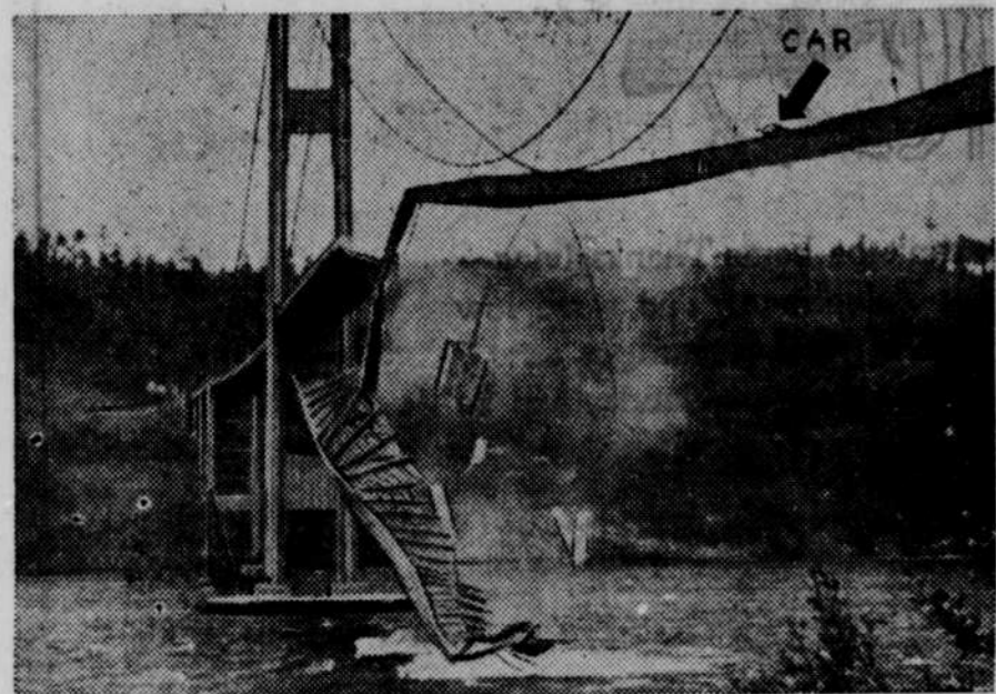
This soundphoto shows the new Narrows bridge at Tacoma, Wash., third longest single suspension span in the world, as it started to disintegrate and fall 190 feet into Puget Sound. The bridge was completed last July at a cost of $6,400,000. Note the car on the bridge which was abandoned by its occupants as the bridge began to collapse.
