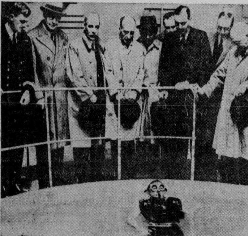
Members of the British parliament, investigating the loss of the submarine Thetis in Liverpool bay, saw a working demonstration of the Davis escape lung recently when they visited the submarine Triumph, sister ship of the ill-fated Thetis. An instructor is shown wearing the lung after he had escaped from a flooded hatch in a demonstration tank.
